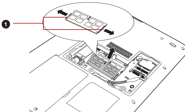
Figure 3-7 Removing the memory module
